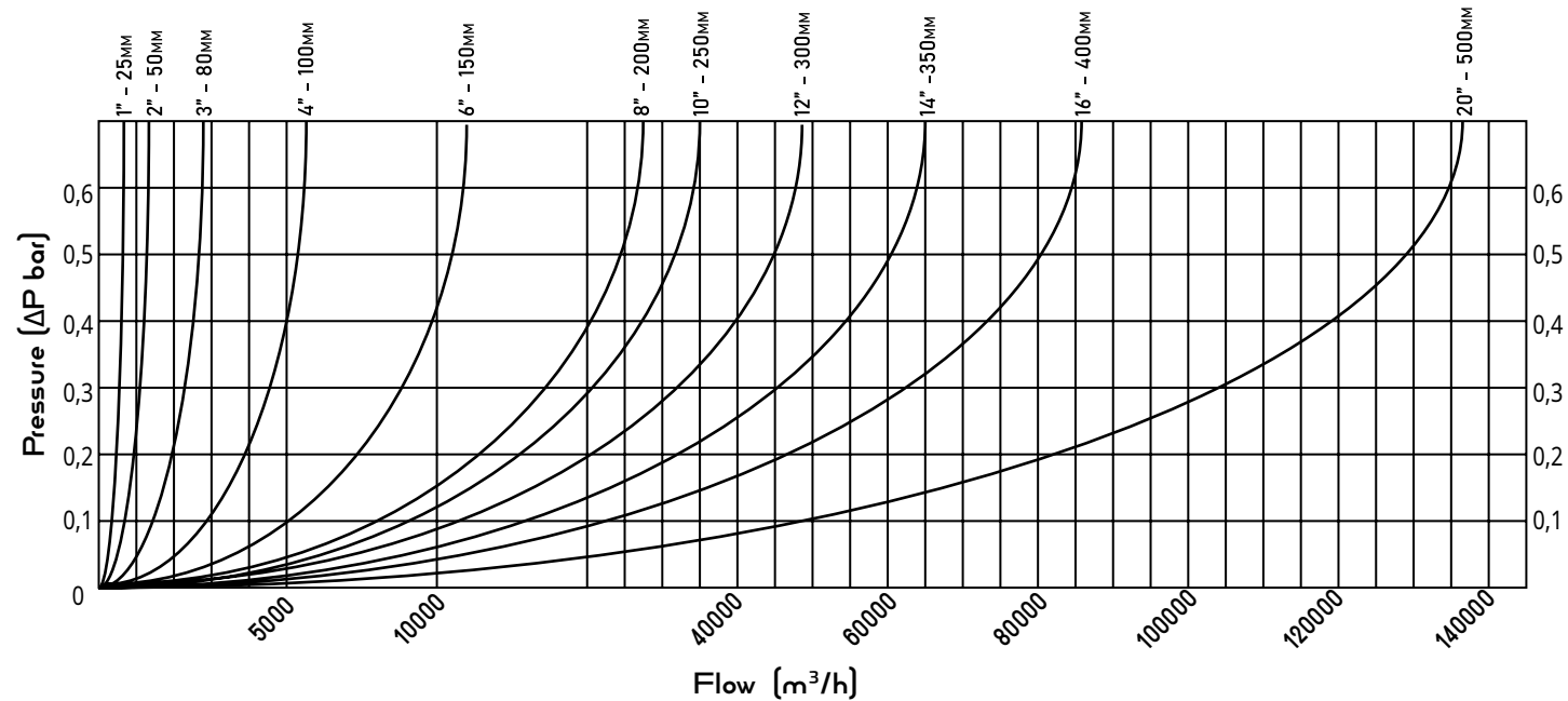
Nominal Air Release Capacity of Non-Pulse Dynamic Air Release Valve
